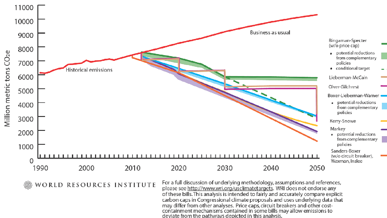
Figure 1. Emissions reductions that would have been required under the climate change bills that were introduced in the 110th U.S. Congress.
